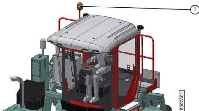
Fig. 14: Gyrophare
