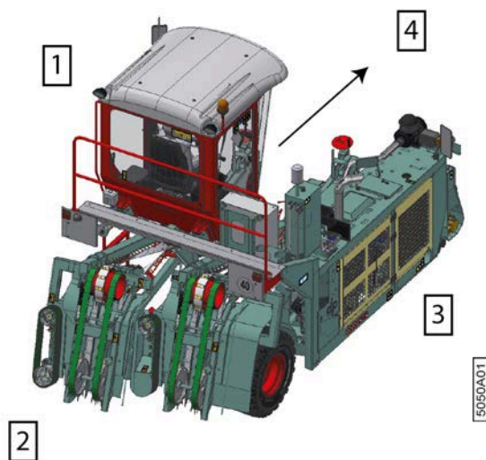
Fig. 7: Direction
