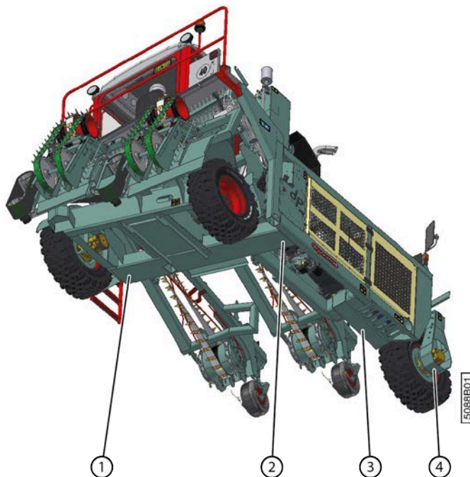
Fig. 122: Points de support
